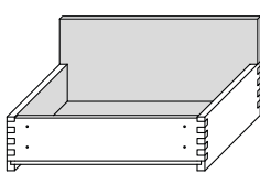
BEH2 With higher drawer back piece (80 mm) for rail; width: drawer external dimensions
