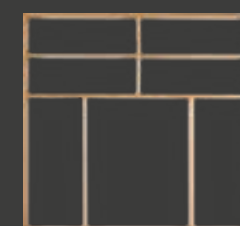
Type U4: height 55 mm or 95 mm Depth 340 - 550 mm / width 350 - 650 mm
