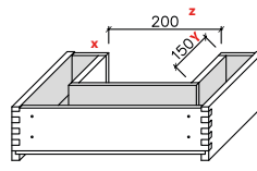
Siphon cutout Fixed 200 x 150 mm centre; variable stating the 3 dimensions x/y/z
